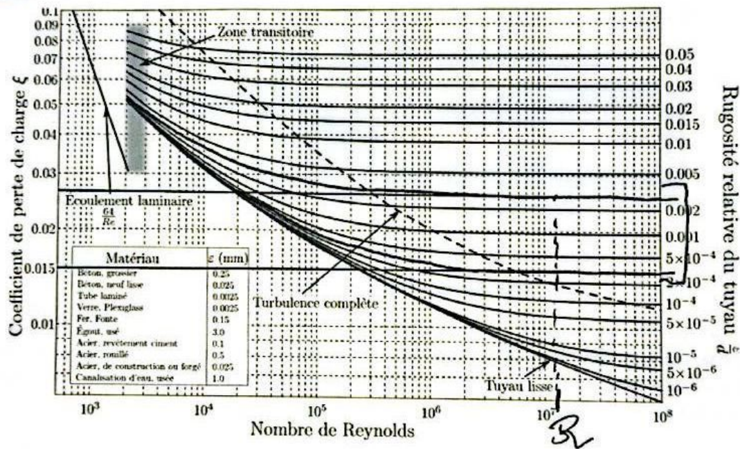
FIGURE 3 – Diagramme de Moody
